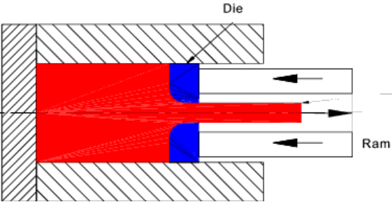
Indirect Extrusion
